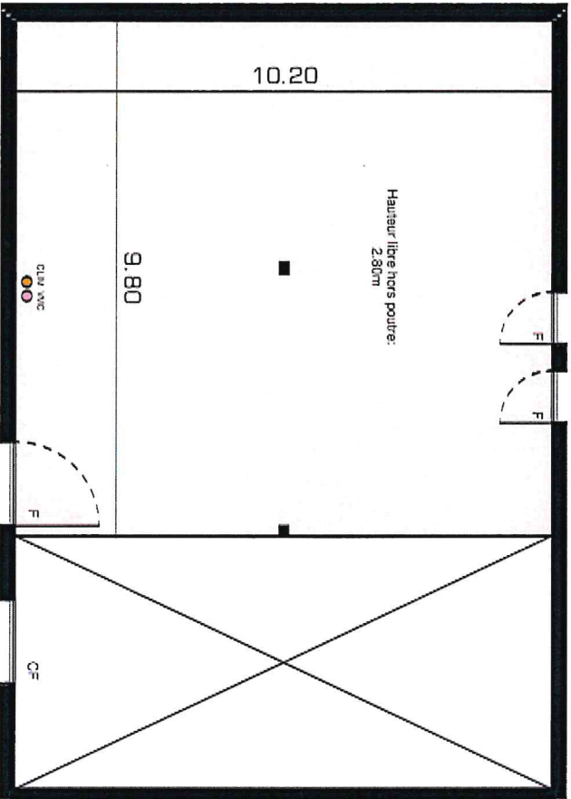
PLAN MEZZANINE
