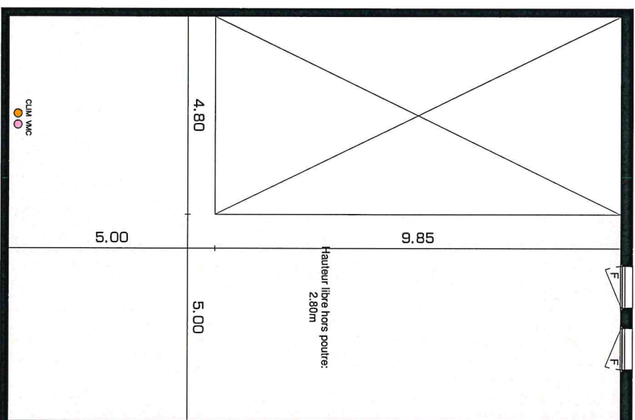
PLAN MEZZANINE
